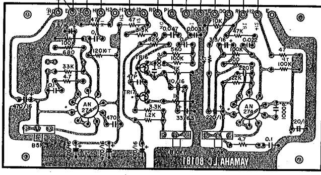
RHP CIRCUIT BOARD
