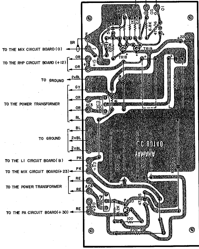
POW CIRCUIT BOARD
